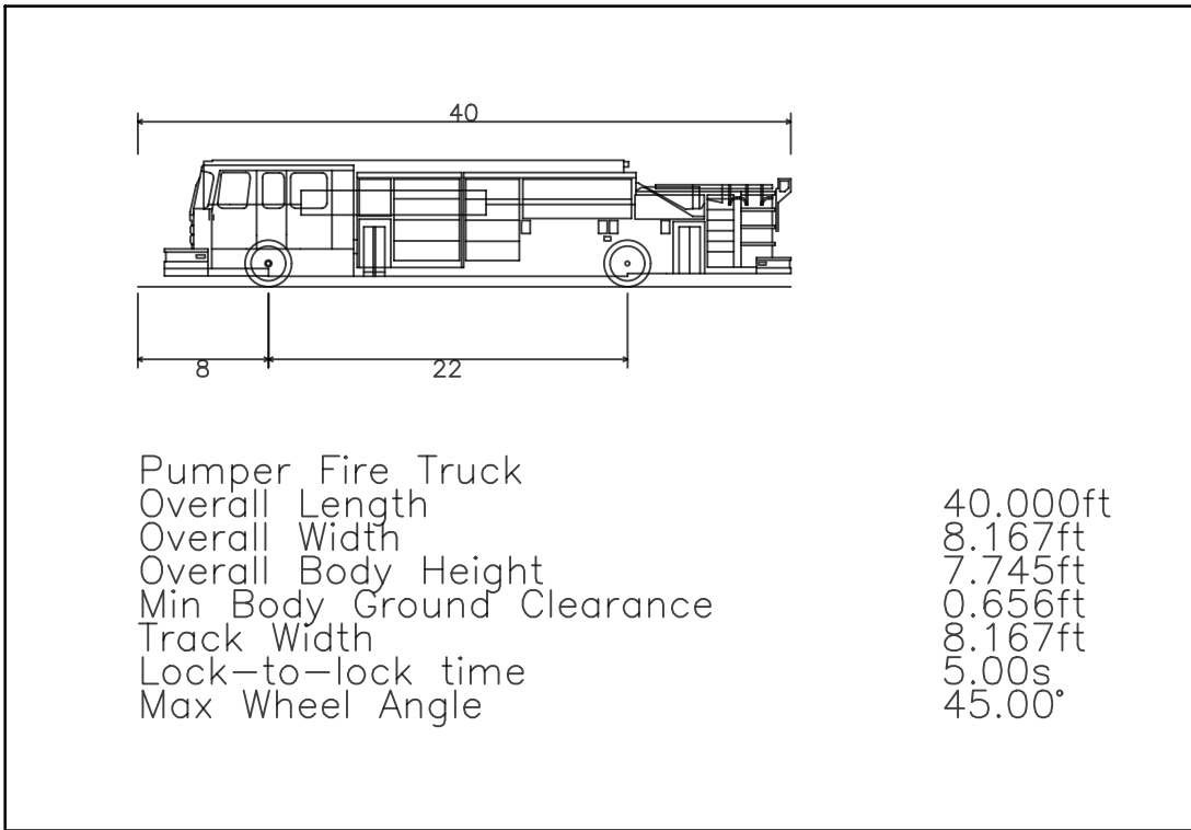
PUMPER FIRE TRUCK DETAIL NOT TO SCALE
